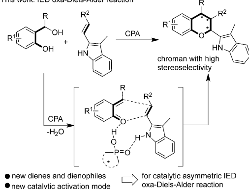
Scheme 3. Design of a catalytic asymmetric IED oxa-DA reaction of in situ generated o -QMs and 3-methyl-2-vinylindoles.
